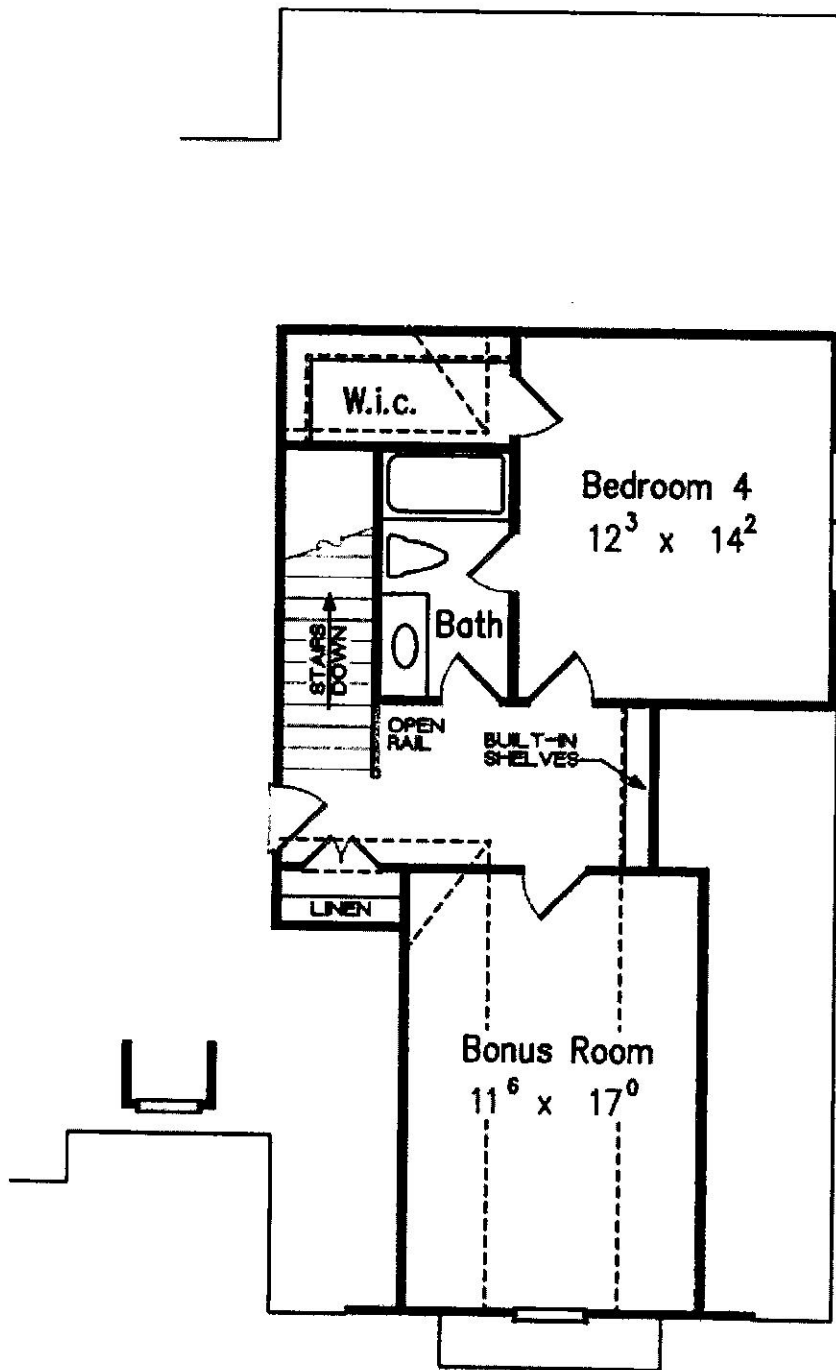
OPT. SECOND FLOOR PLAN
