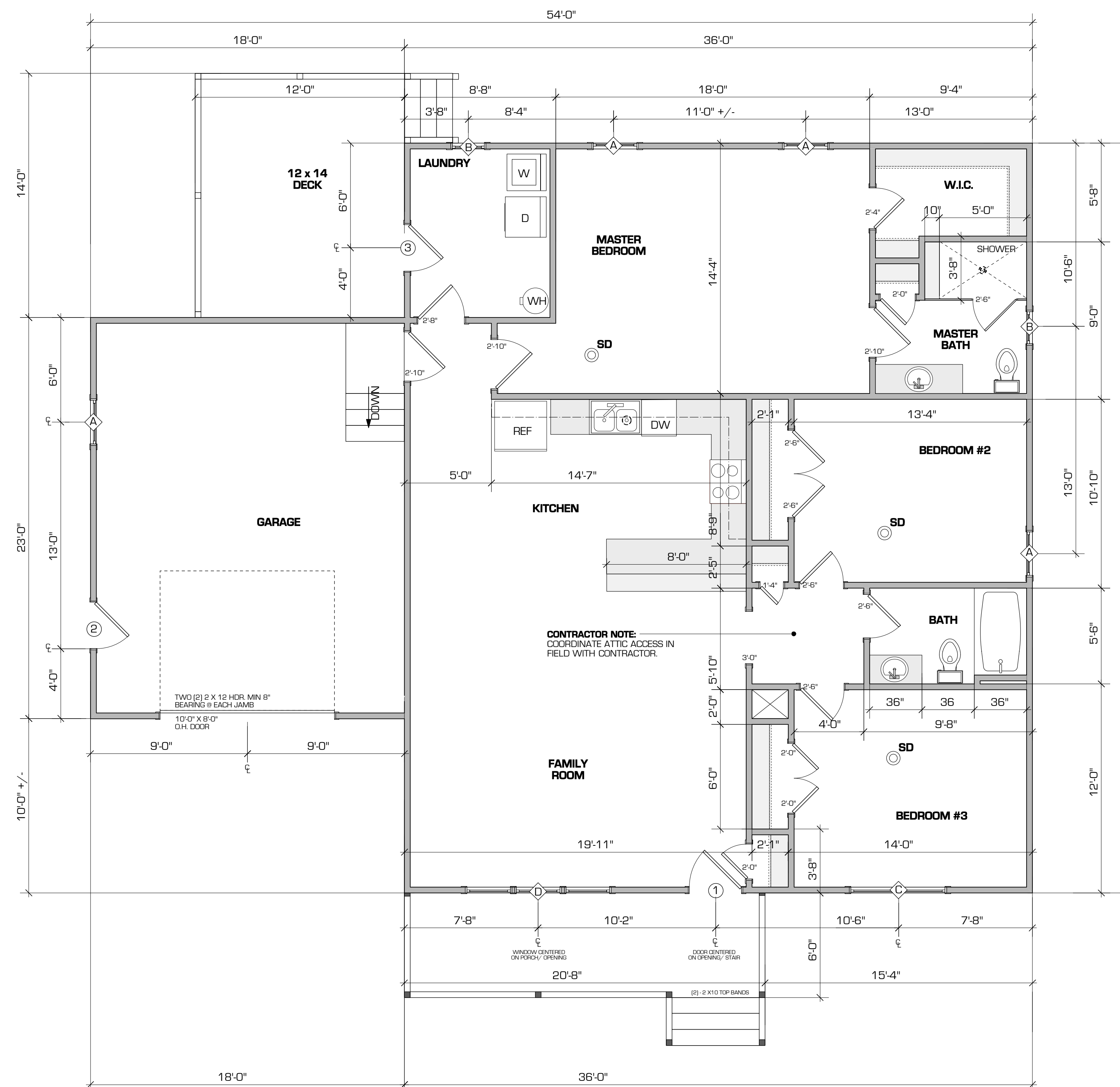
Floor Plan 1 1/4" = 1'-0" PLAN NORTH
